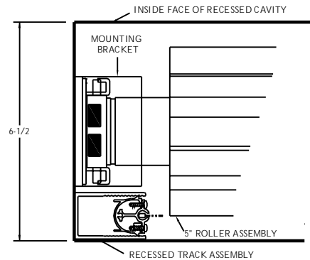
RELATIONSHIP OF U-CHANNEL TO MOTOR BRACKET IN A MINIMUM RECESSED CAVITY C/W 5" ROLLER
